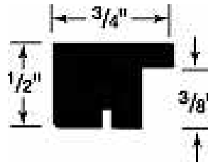
Profile 11 (End View)
