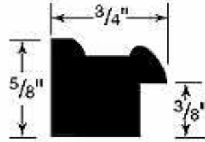
Profile 30 (End View)
