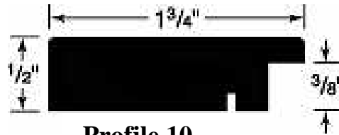
Profile 10 (End View)
