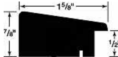
Profile 21 (End View)
