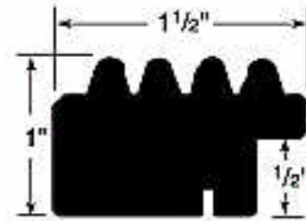
Profile 25 (End View)
