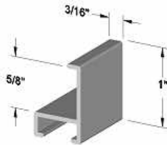
Profile 85 (End View)
