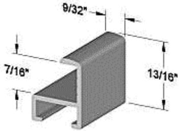
Profile # 78 (End View)
