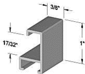
Profile 84 (End View)
