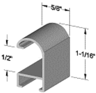
Profile 74 (End View)
