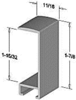
Profile # 82 (End View)
