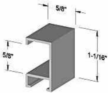
Profile 73 (End View)
