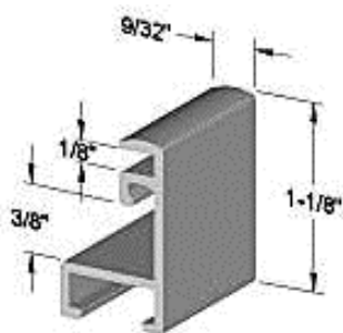
Profile # 81 (End View)
