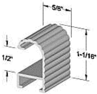
Profile 75 (End View)
