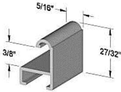
Profile 77 (End View)
