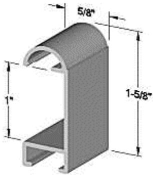
Profile # 82 (End View)
